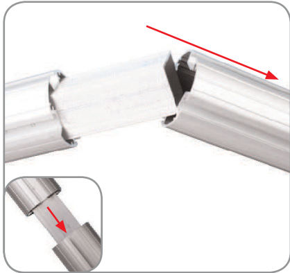
Align and slide female post over male post.
