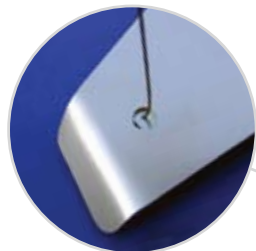
Simply push the cable grip through the hole to connect cable to baseplate
